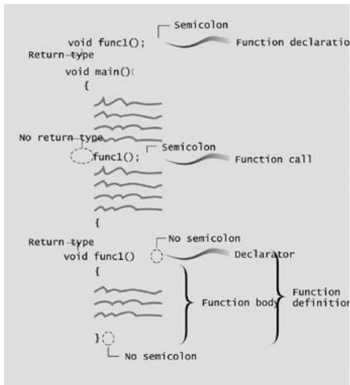
Figure 5.2 Function syntax.
