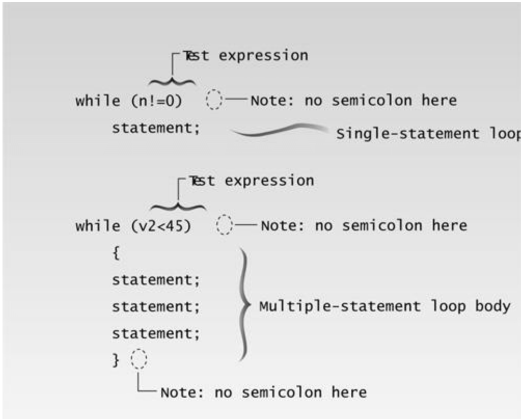
Figure 3.3 Syntax of the while loop.
