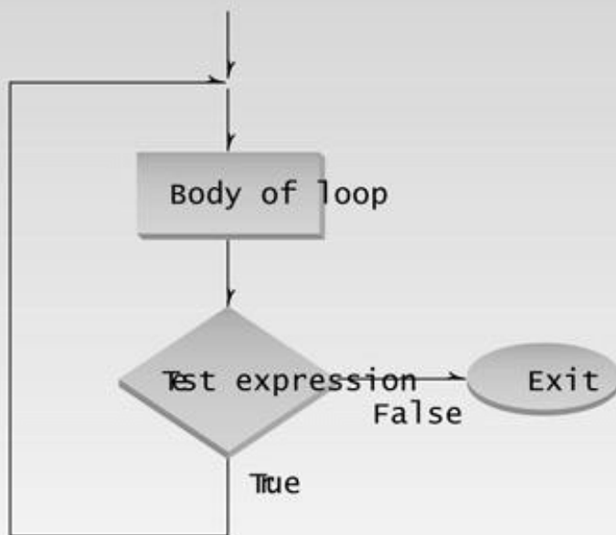
Figure 3.6 Operation of the do loop.
